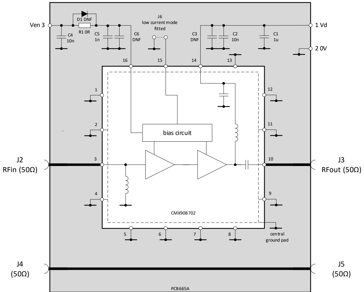
Figure 62: EV90B702 Schematic
