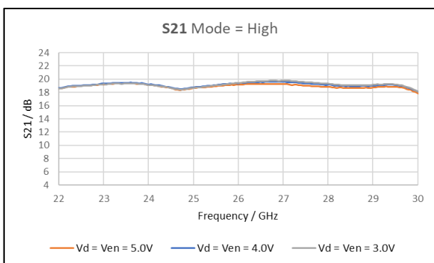
Figure 19: S21 Vd = Ven, low current mode
