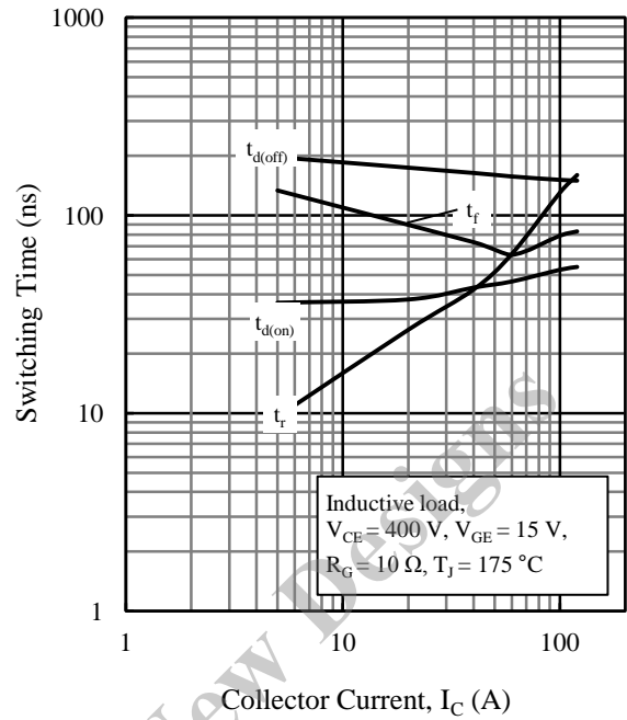
Figure 15. Switching Time vs. Collector Current
