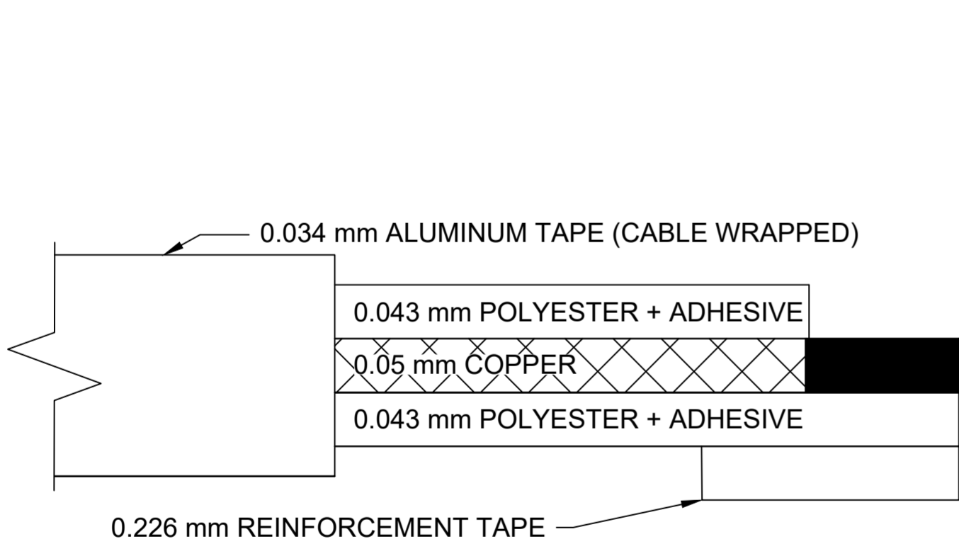
CROSS-SECTION
