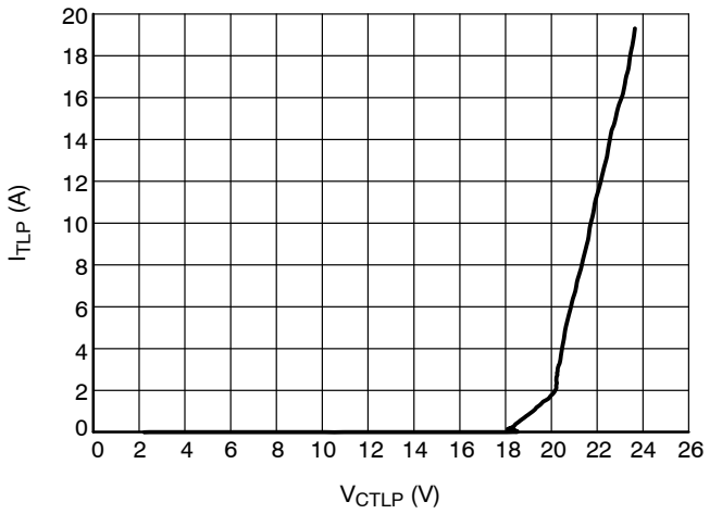
Figure 4. Pin 2 to Pin 1 100 ns TLP I-V Curve
