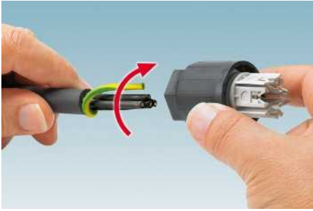
1. Strip the cable and prepare the PE conductor.
