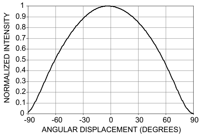
Figure 12: Radiation Pattern
