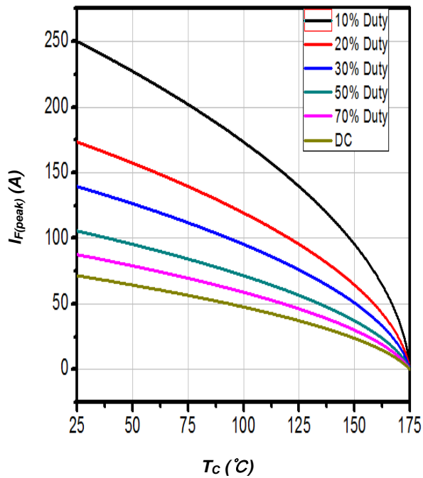
Figure 3. Current Derating
