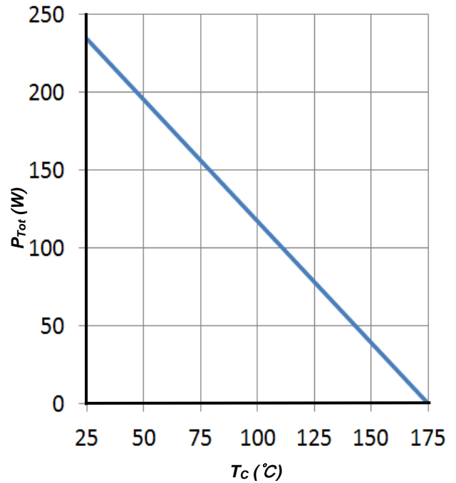
Figure 4. Power Derating
