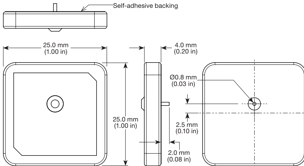
Figure 1. 915-CPA Antenna Dimensions
