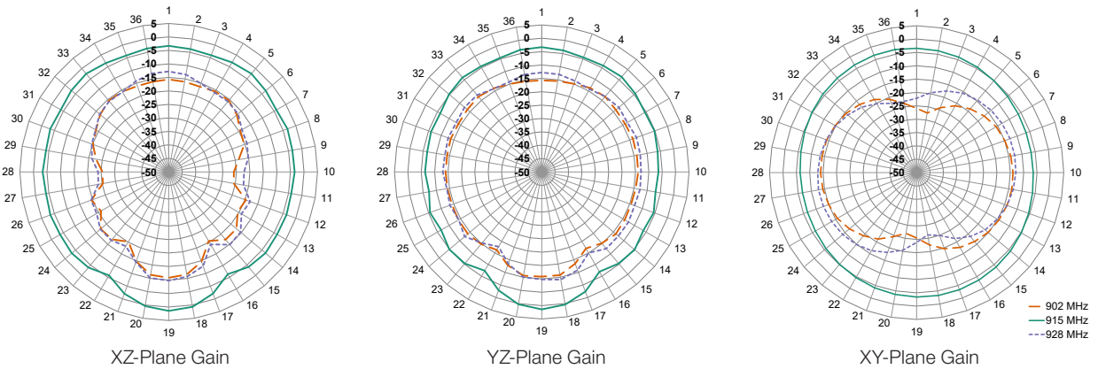
Figure 6. Radiation Patterns for 915-CPA Antenna
