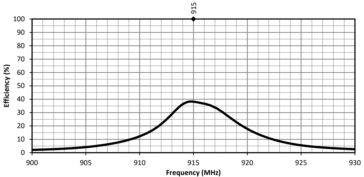
Figure 5. 915-CPA Antenna Radiation Efficiency
