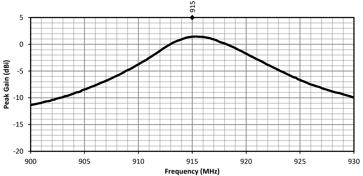
Figure 4. 915-CPA Peak Gain
