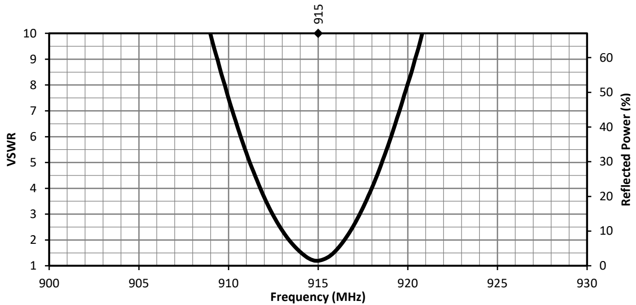
Figure 2. 915-CPA VSWR
