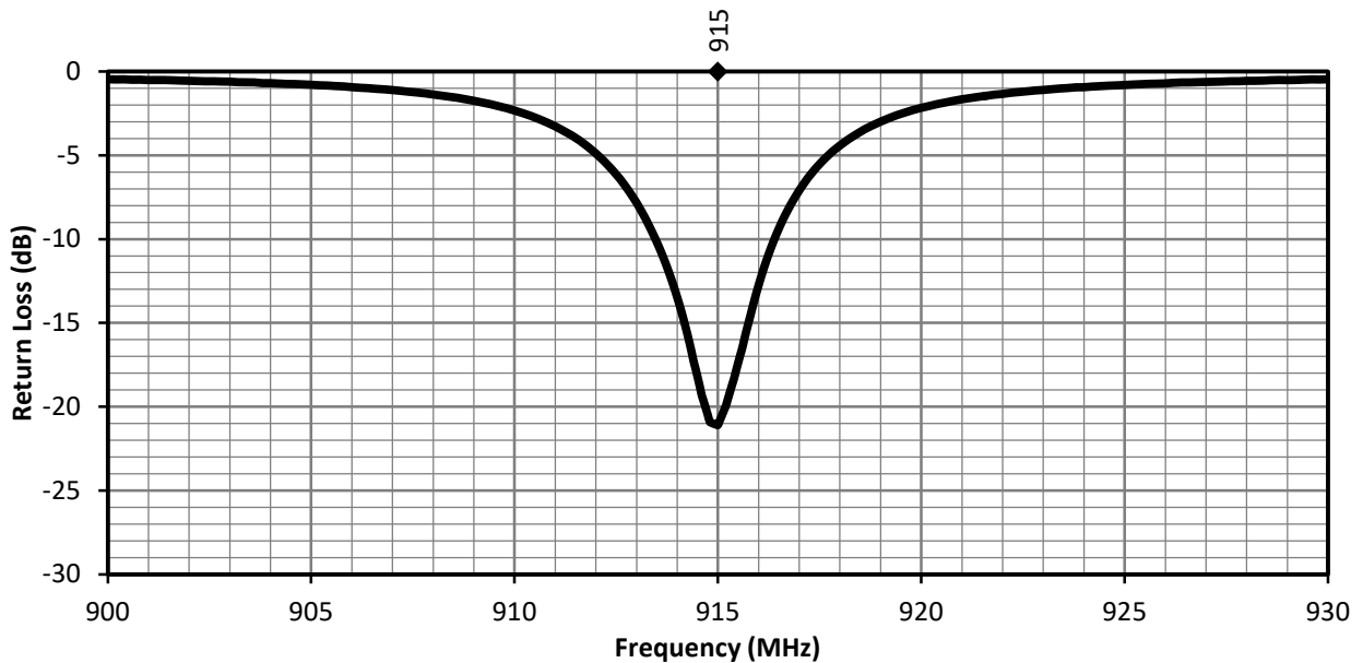
Figure 3. 915-CPA Return Loss
