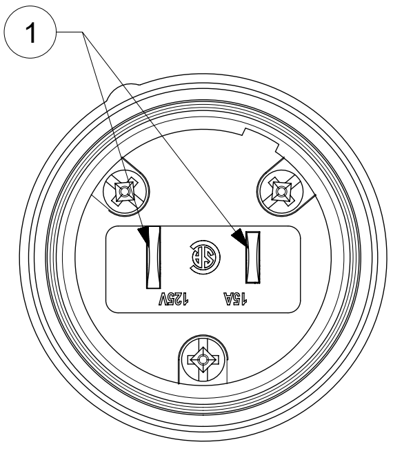
FACE VIEW
