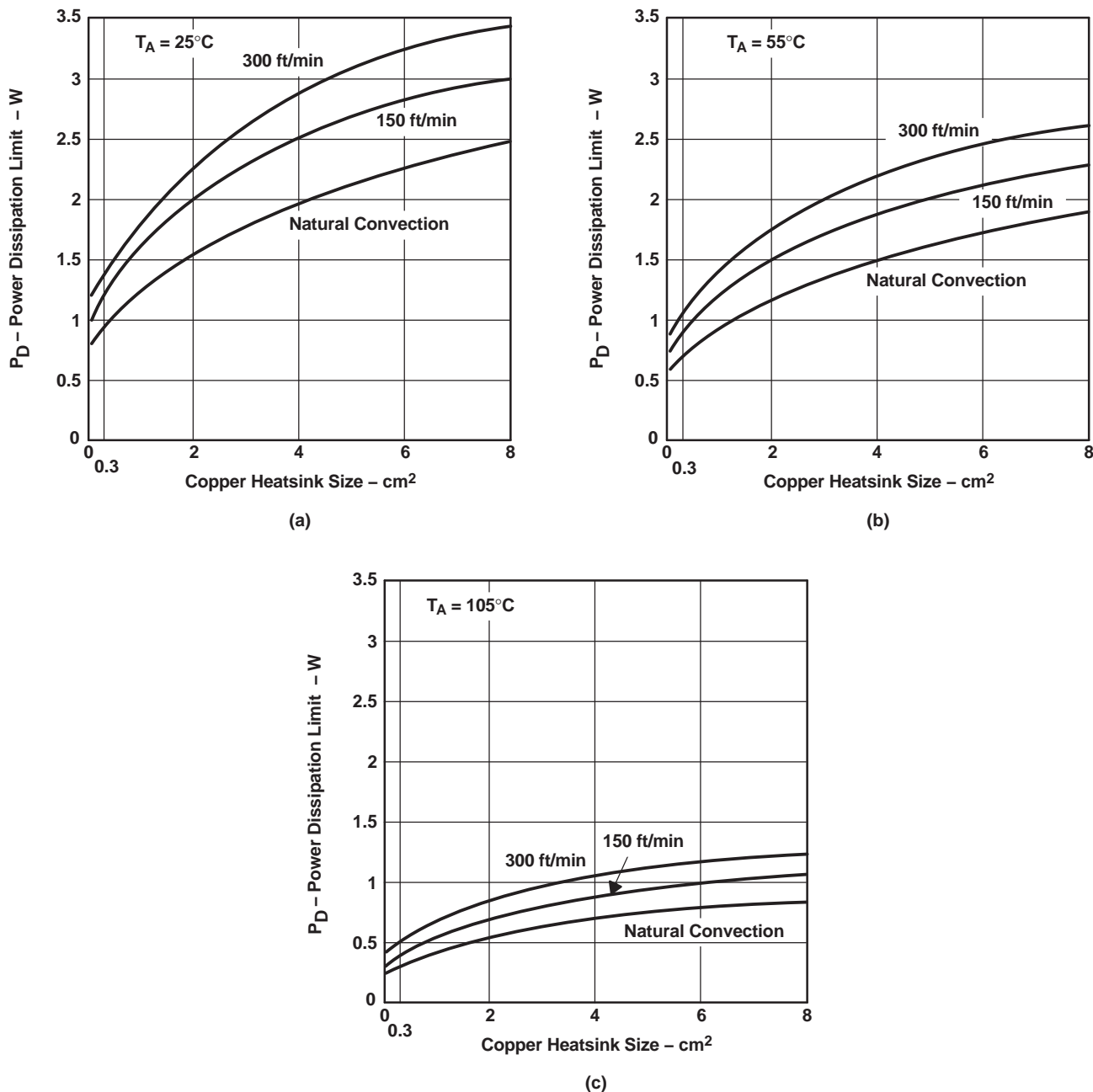
Figure 12. PWP Package Power Ratings at Ambient Temperatures of 25°C, 55°C, and 105°C
