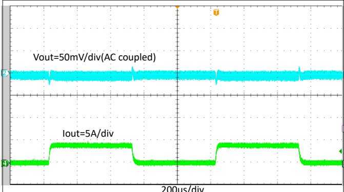
Figure 8-18. TPS564247 Transient Response with 0.1 A to 4 A by 2.5-A/ \mu\text{s} Load Step
