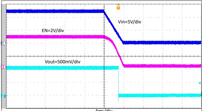
Figure 8-14. Start-Up with V_{IN} Falling, I_{OUT} = 4\text{ A}
