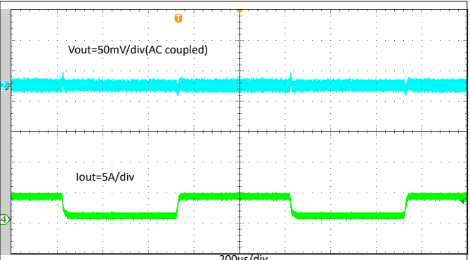
Figure 8-15. TPS564242 Transient Response with 0.4 A to 3.6 A by 2.5-A/ \mu\text{s} Load Step
