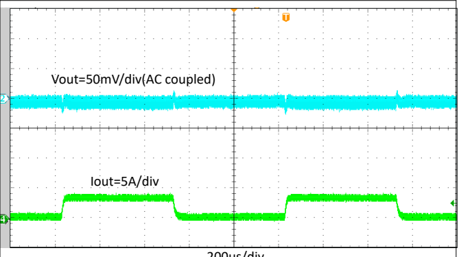
Figure 8-17. TPS564247 Transient Response with 0.4 A to 3.6 A by 2.5-A/ \mu\text{s} Load Step
