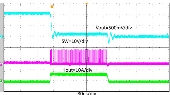
Figure 8-19. TPS564242 Normal Operation to Output Hard Short
