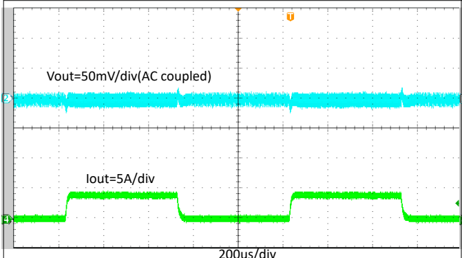
Figure 8-16. TPS564242 Transient Response with 0.1 A to 4 A by 2.5-A/ \mu\text{s} Load Step
