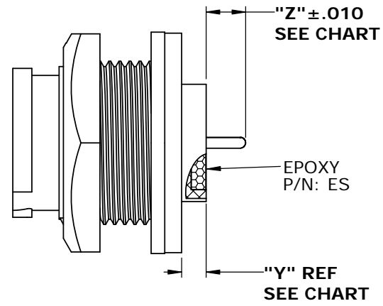
ASSEMBLED VIEW W7281-2SG-P-3ES SHOWN
