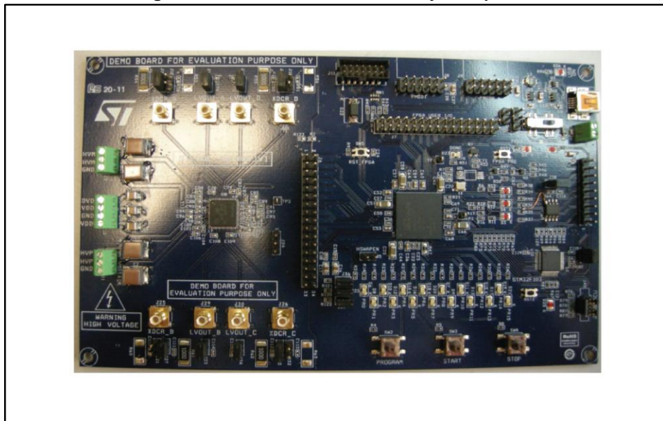
Figure 1: STEVAL-IME003V1 board layout top view
