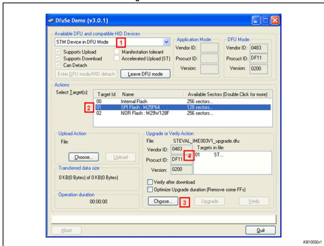
Figure 2: DfuSe GUI
