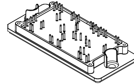
PIM53, 93x47 (SOLDER PIN) CASE 180CC
