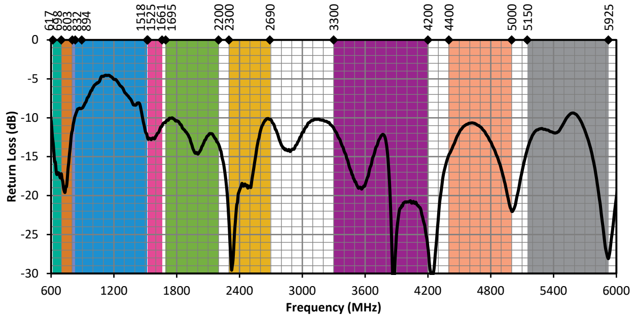
Figure 5. ANT-5GWWS6-SMA Return Loss, Straight
