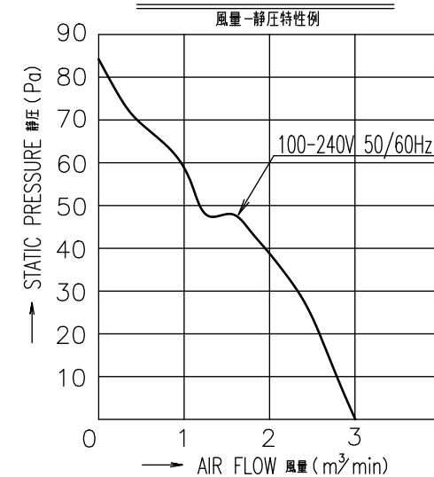
PERFORMANCE CURVES
