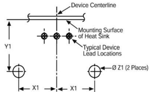
Mounting Details:
