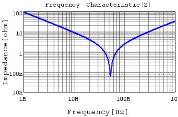
RCE5C2E182J1K1H03B |Z| DC0V, 25degC
