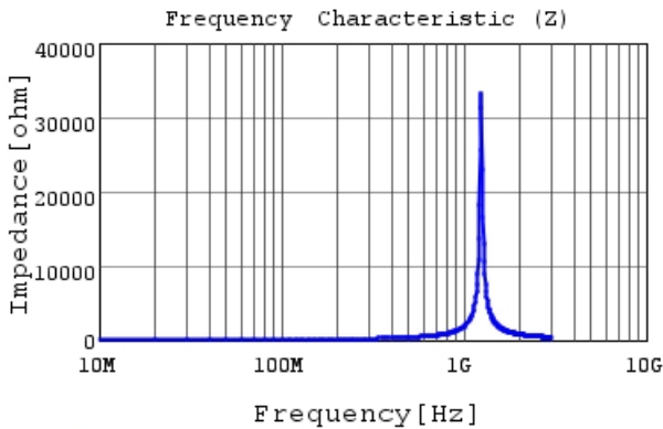
LQG15WZR11J02 |Z|
