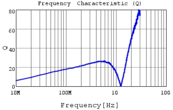
LQG15WZR11J02 Q
