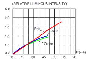
FIG.2 RELATIVE LUMINOUS INTENSITY VS. FORWARD CURRENT
