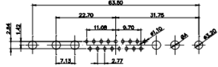
21W4 Male/Female
