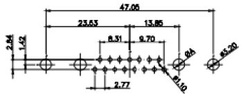
17W2 Male/Female
