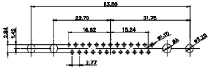
27W2 Male/Female
