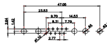
13W3 Female
