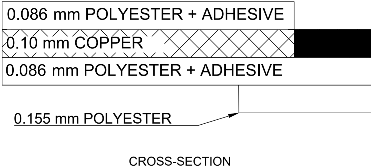
CROSS-SECTION
