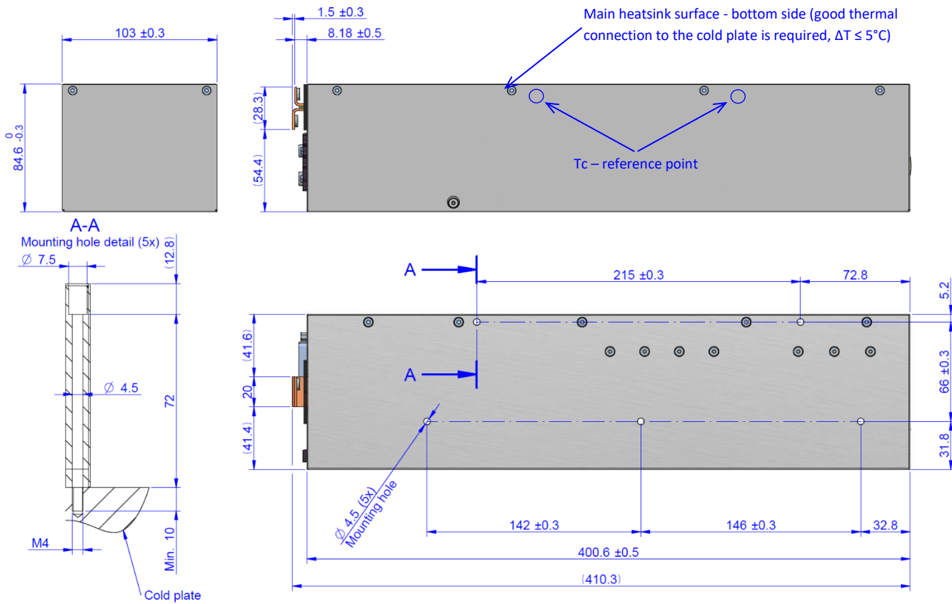
Figure 2. Mechanical Dimensions
