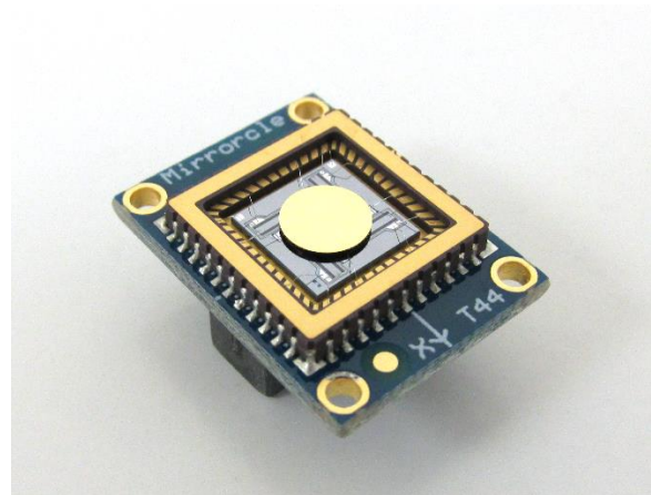
Figure 1. Image of the A8L2.2-5000AU-TINY48.4 device shown without any window (open cavity). The 5mm mirror is gold-coated for optimized performance in near-IR and IR wavelengths. The connectorized package "TINY48.4" is 15mm x 20mm x 9mm
