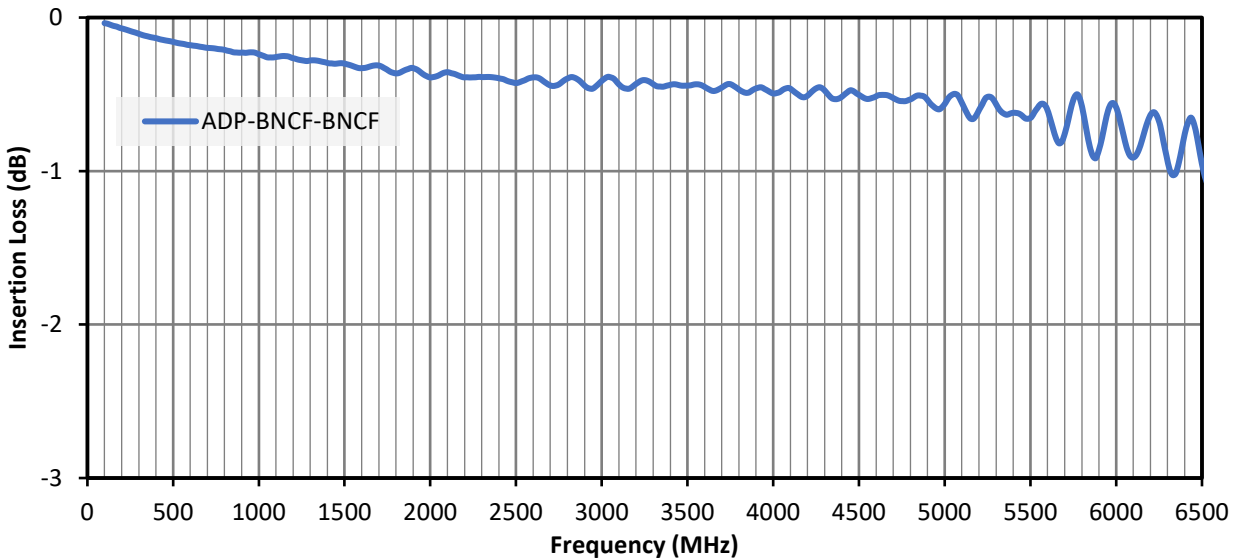
Figure 2. Insertion Loss for the ADP-BNCF-BNCF Adapter
