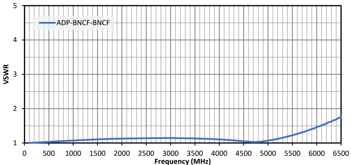
Figure 3. VSWR for the ADP-BNCF-BNCF Adapter
