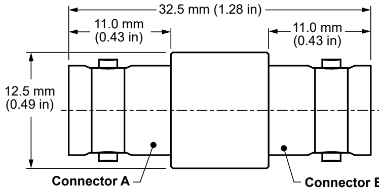
Figure 1. Product Dimensions for the ADP-BNCF-BNCF Adapter
