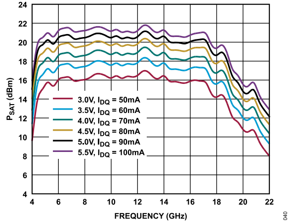
Figure 40. P_{SAT} vs. Frequency for Various Supply Voltages and I_{DQ} Values, 4 GHz to 22 GHz, R_{BIAS} = 392 \Omega
