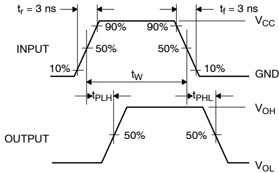
Figure 6. AC Waveforms
