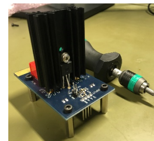
Step 6 Heatsink mounting
