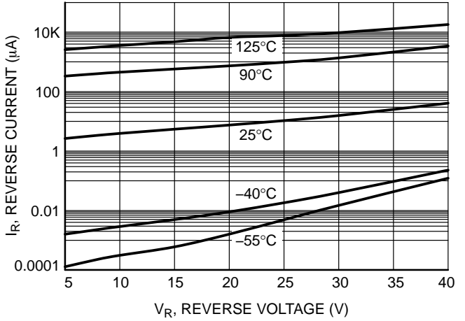
Figure 6. Leakage Current
