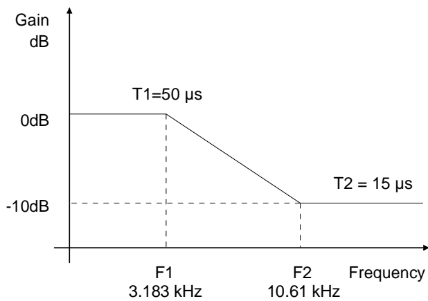
Figure 6. De-Emphasis Curve
