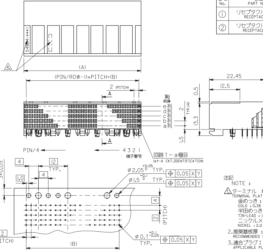
基板穴推奨寸法 (部品実装) RECOMMENDED P.C.B. LAYOUT (COMPONENT SIDE)
