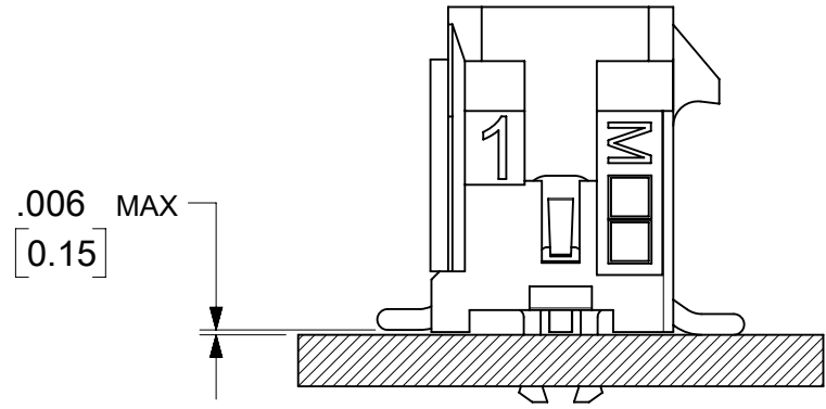
COPLANARITY DETAIL SEE NOTE #7
