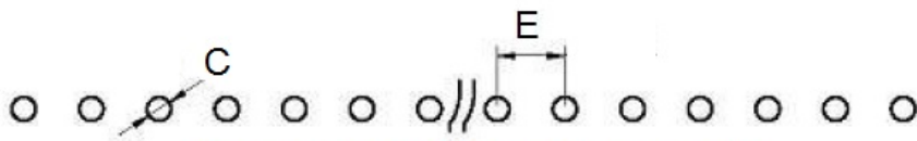
Recommended PCB Hole Layout
