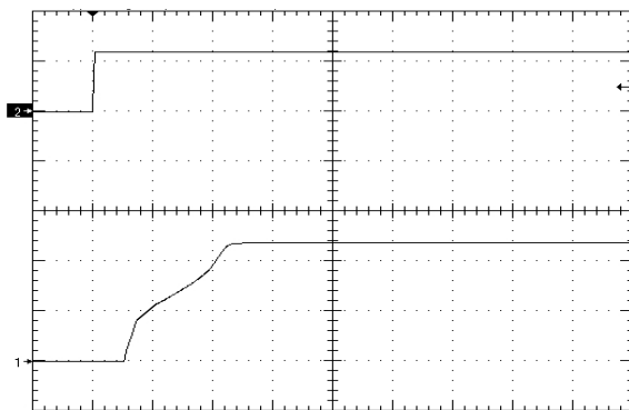
Figure 11. Startup Waveform via Enable Pin, time scale 10mS/div. Vin=Vin_nom, Iout=full load Cout=0uF, Ch1=Vout (5V/div), Ch2=enable (5V/div)
