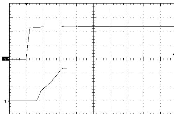
Figure 10. Startup Waveform via Input Voltage, time scale 10mS/div. Vin=Vin_nom, Iout=full load Cout=2000uF, Ch1=Vout (5V/div), Ch2=Vin (10V/div)
