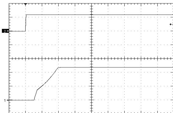
Figure 9. Startup Waveform via Enable Pin, time scale 10mS/div. Vin=Vin_nom, Iout=no load Cout=0, Ch1=Vout (5V/div), Ch2=enable (5V/div)
