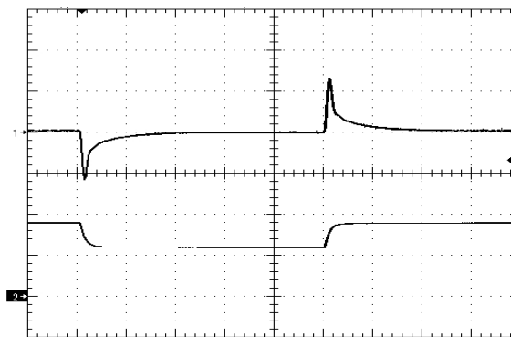
Figure 12. Load Transient Response (50mV/div), di/dt=0.1A/uS, 50%-75%-50% of full load, Cout=Fig16 time scale: 200uS/div. Ch1=Vout, Ch2=Iout (1A/div)
