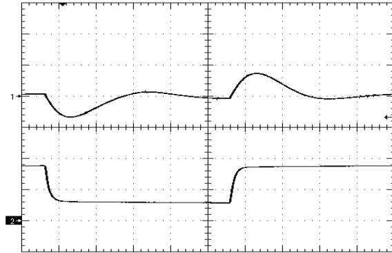
Figure 14. Load Transient Response 50mV/div, di/dt=0.2A/uS, 25% - 75% - 25% of full load +2000uF low ESR Oscon, time scale: 200uS/div. Ch1=Vout, Ch2=Iout (1A/div)
