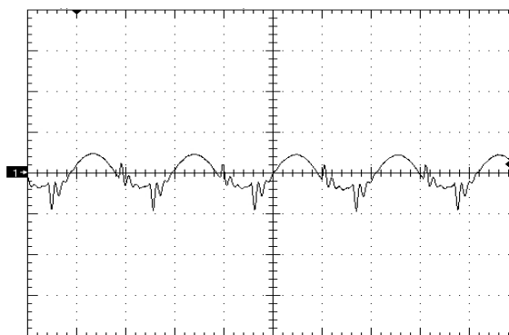
Figure 8. Output Voltage Ripple (20mV/div), time scale – 1uS/div. Vin=Vin_nom, full load Cout=0.1uF ceramic + 10uF Tantalum (see Fig 16)
