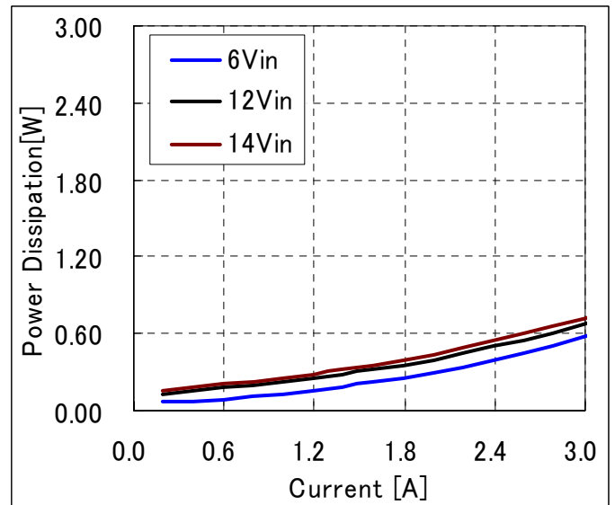
Fig-1.0V-3: Power dissipation vs. load current and input voltage for V_{out}=1.0V . Airflow rate=200 LFM (1m/s) and T_a=25^{\circ}C .
