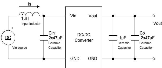
Fig. D: Test setup for measuring output voltage ripple
