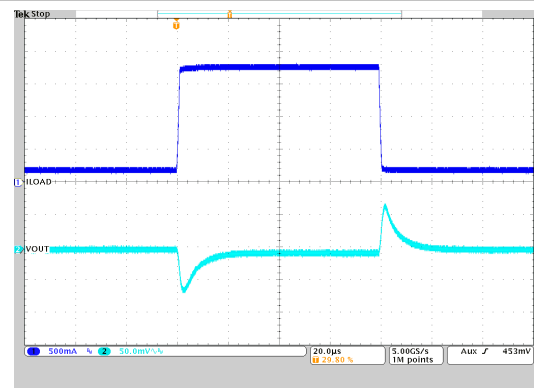
Figure 10-29. Load Transient Response
