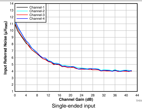
Figure 14. Input-Referred Noise vs Channel Gain Single-ended input
