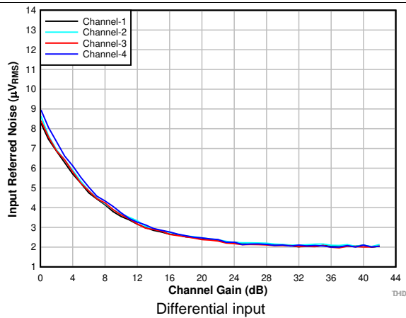
Figure 13. Input-Referred Noise vs Channel Gain Differential input
