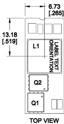
Figure 34. Pick and Place Location.
