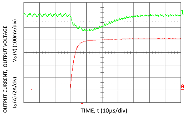
Figure 12. Transient Response to Dynamic Load Change from 50% to 100% of full load ( V_o = 3.3 Vdc, C_{ext} = 2 \times 150 µF Polymer Capacitors).
