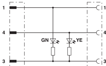
Contact assignment of M12 plugs / M8 sockets
