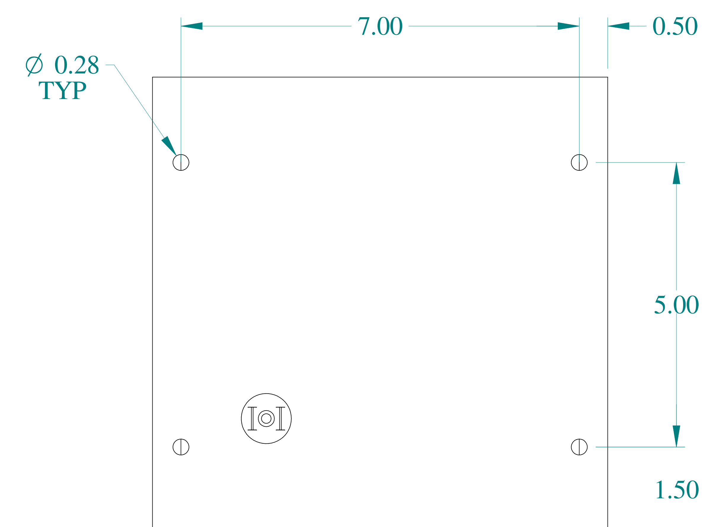
BOTTOM VIEW
