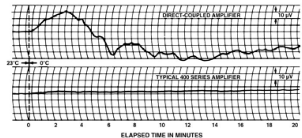
FIG. 2 EFFECT OF ABRUPT TEMPERATURE CHANGE
