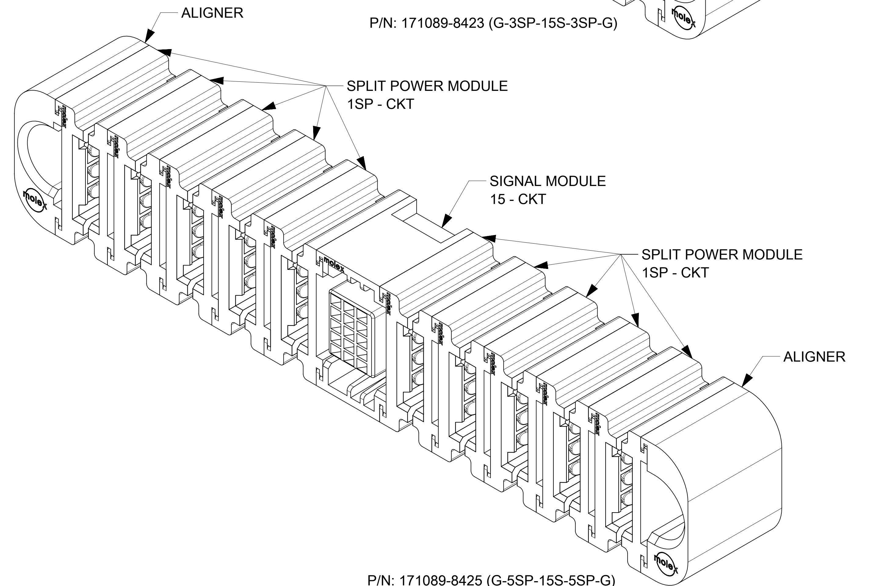
P/N: 171089-8425 (G-5SP-15S-5SP-G)
