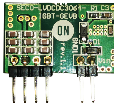
Figure 1. Board Layout
