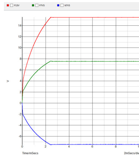
Figure 17. Output Voltages for V_{in} = 15\text{ V}
