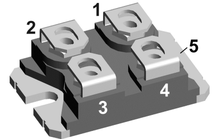
Backside: cathode
