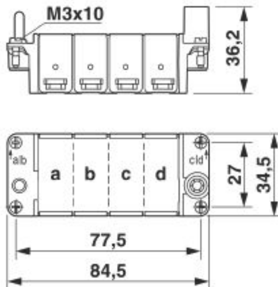
Dimensional drawing
