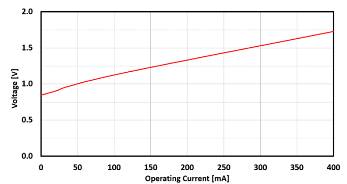
FIG. 14: SLED 3 FORWARD VOLTAGE VS CURRENT
