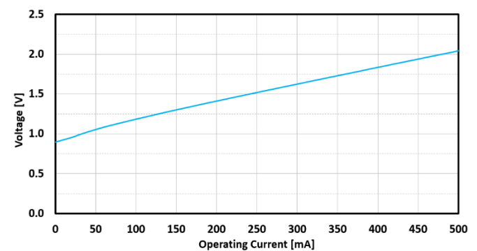
FIG. 16: SLED 5 FORWARD VOLTAGE VS CURRENT
