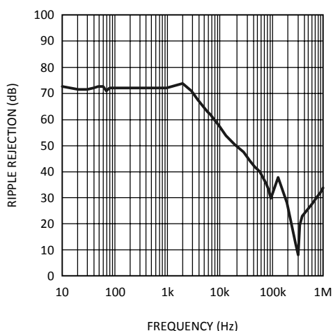
Figure 8. Ripple Rejection
