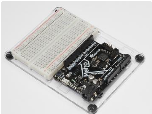
Adafruit Metro (or Metro Express) + Breadboard + Mounting Plate If you have not assembled this, we have a handy guide! ( link )
