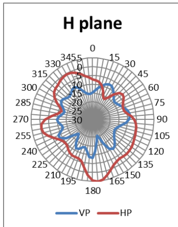
Radiation pattern, 2400 MHz
