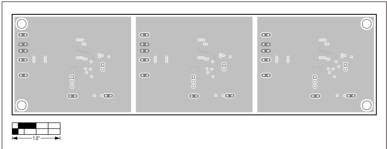
MAX17640A/MAX17640B/MAX17640C EV Kits PCB Layout Diagram—Layer 2
