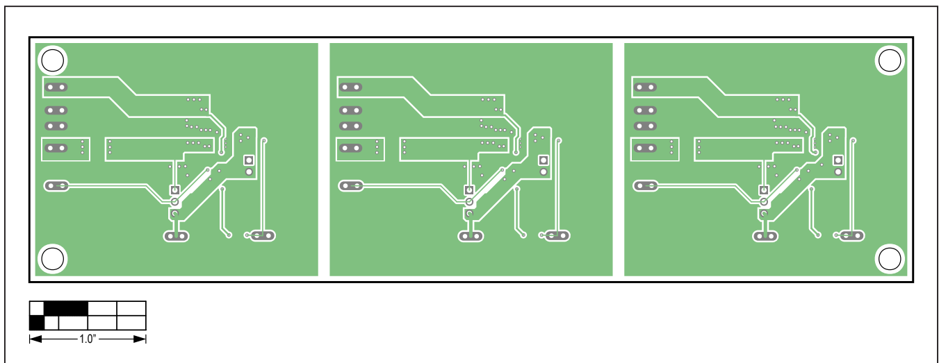
MAX17640A/MAX17640B/MAX17640C EV Kits PCB Layout Diagram—Layer 3
