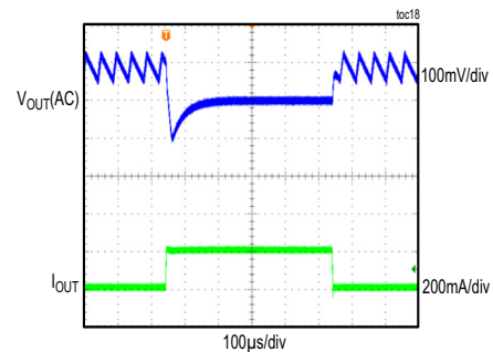
MAX17640B LOAD TRANSIENT RESPONSE
